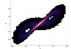
(g) BFloat16sr
