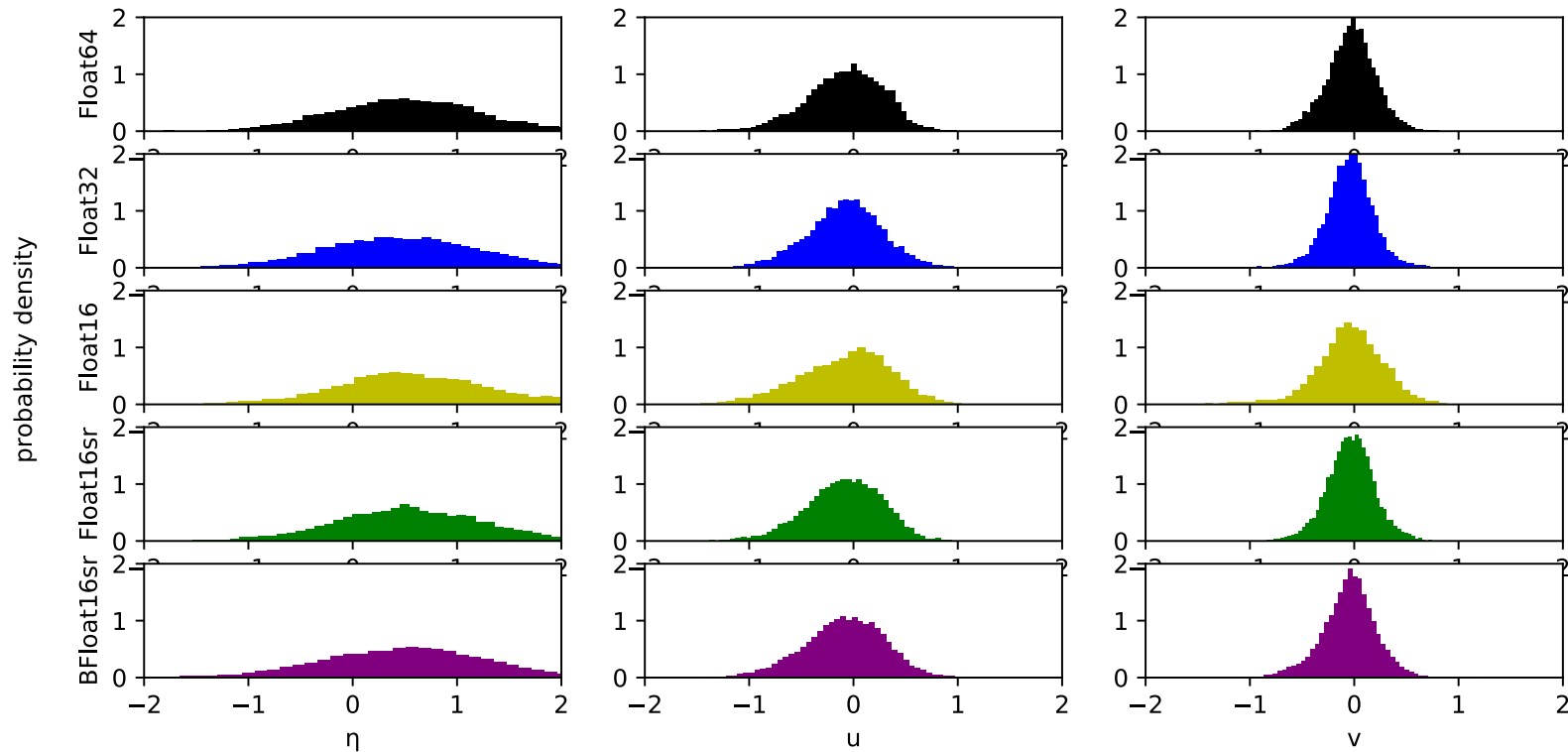
Model climatology for Shallow Water Equations after single 20 year run (values spatially averaged over (lon,lat) \in (100, 200)km \times (400, 500)km region)
