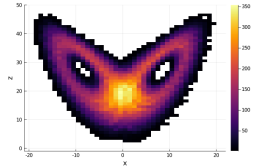
(e) Float16sr
