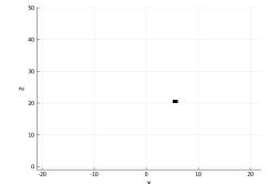
(f) BFloat16
