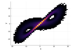
(e) Float16sr
