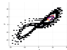
(f) BFloat16
