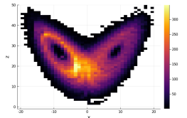
(g) BFloat16sr
